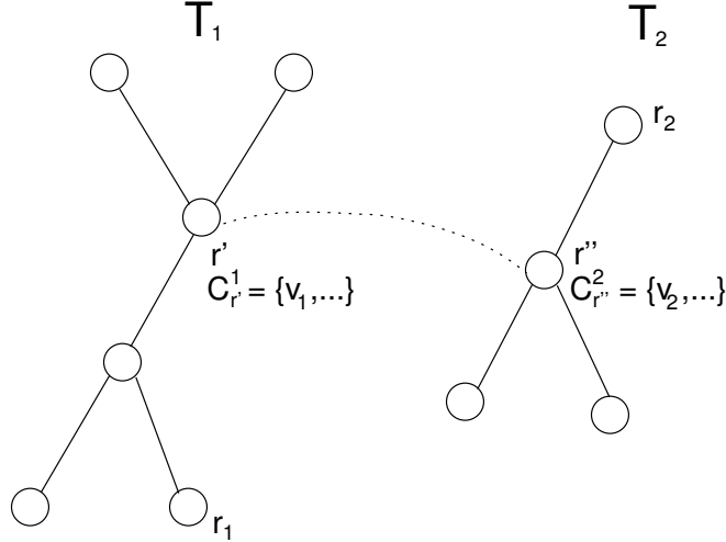
Figure 4: T_1 and T_2 have been recursively computed by GOMORYHUALG. Then we find r' and r'' such that v_1 (the shrunken vertex corresponding to V \setminus W in T_1 ) is in the partition of r' , and similarly for r'' and v_2 . Then, to compute T , we connect r' and r'' , and recompute the partitions for the whole tree according to COMPUTEPARTITIONS.
